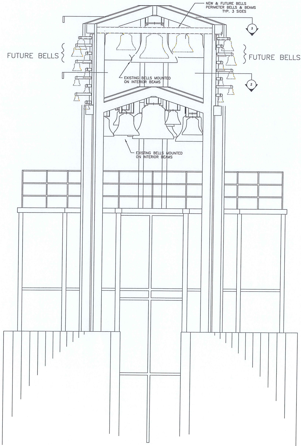
1 Elevation 3/8" = 1' 0"
